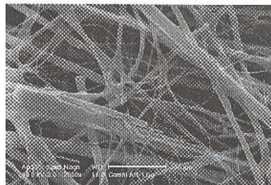
Figure 4. "Boron free" glass fiber media from a unused Absolute filter.
