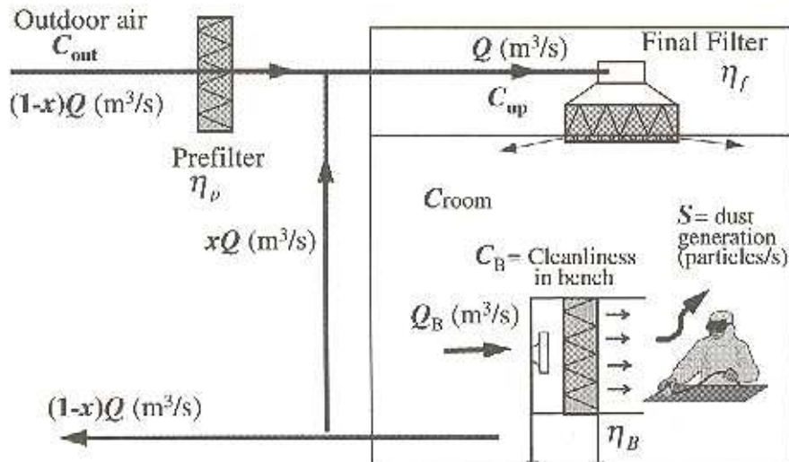
DIAGRAM 9. UNIDIRECTIONAL FLOW BENCHES - Cleanliness calculation
