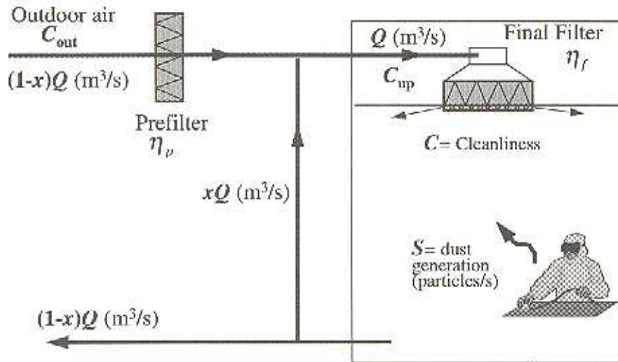
DIAGRAM 8. NONUNIDIRECTIONAL FLOW SYSTEM - Cleanliness calculation
