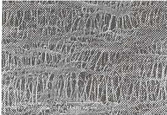
Figure 4. Example of PTFE filter media.
